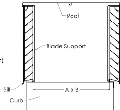
Section View
