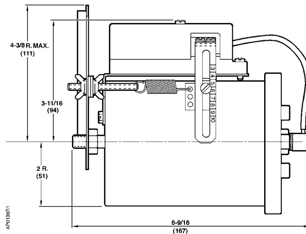
Figure 8. No. 3 Actuator with the RL 147 Positioning Relay Mounted Dimensions. Dimensions are in Inches (Millimeters).
